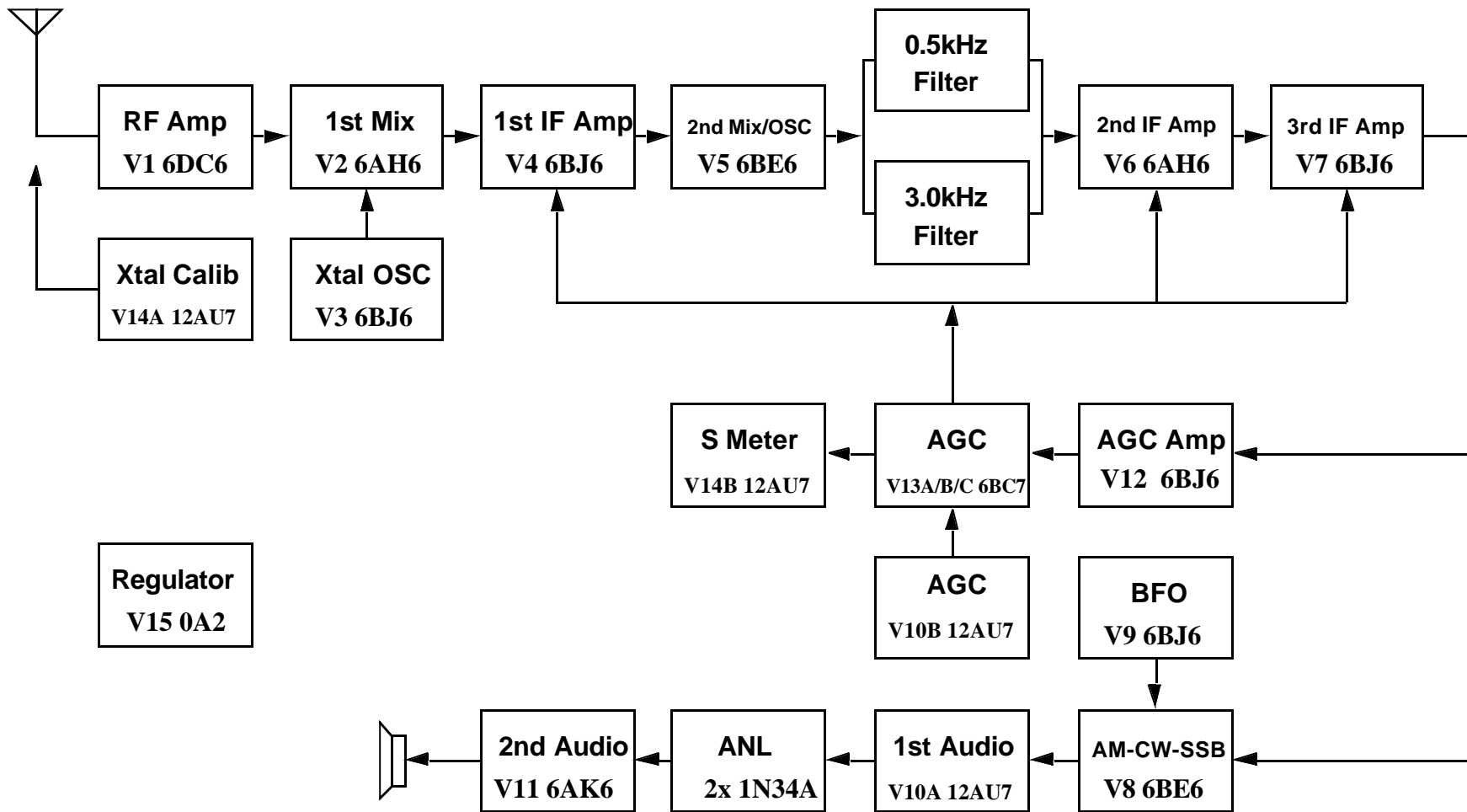
Block Diagram of the DX Communication Receiver : Radio Handbook 16th Edition
